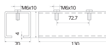
Top track connector Code: 450-47911
