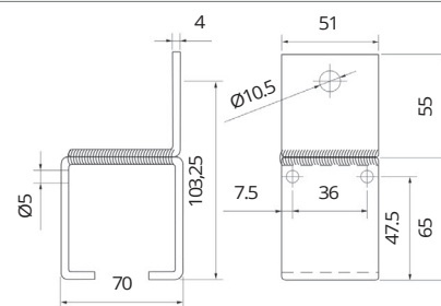
Face fix bracket Code: 450-47950
