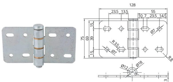
Steel middle hinge Code: 303-314
