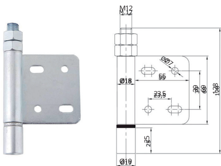
Steel End Hinged Bottom Guide Code: 303-311
