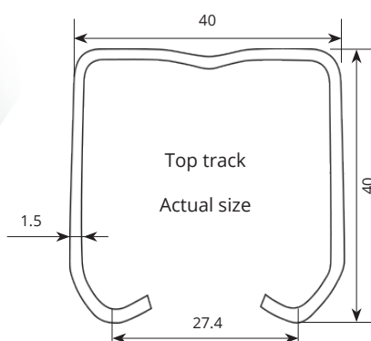
3M Top track Code: 303-303-3
