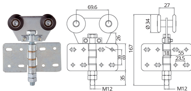
Steel middle hinged double axle hanger 70kg capacity Code: 303-312
