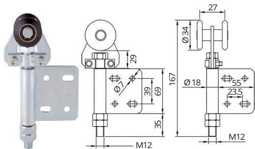
Steel end hinged hanger, 70kg capacity Code: 303-310
