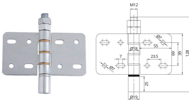
Steel Middle Hinged Bottom Guide Code: 303-313
