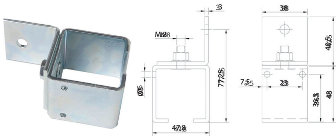
Bracket with bolt Code: 303-307
