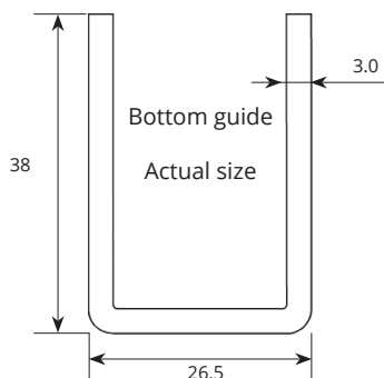
3M Bottom track Code: 303-302-3
