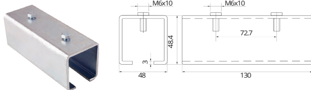
Track connector Code: 303-308
