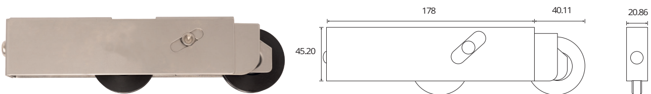
Stainless Steel twin roller unit - 300kg capacity (Maximum Adjustment: 218mm) Code: 100-203
