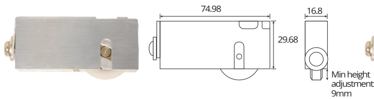
Single nylon roller unit - 25kg capacity (Maximum Adjustment: 93mm) Code: 100-200
