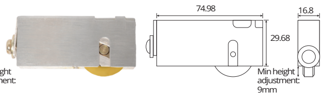
Single brass roller unit - 35kg capacity (Maximum Adjustment: 93mm) Code: 100-201
