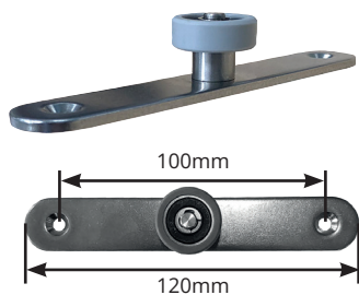
Single bearing guide
